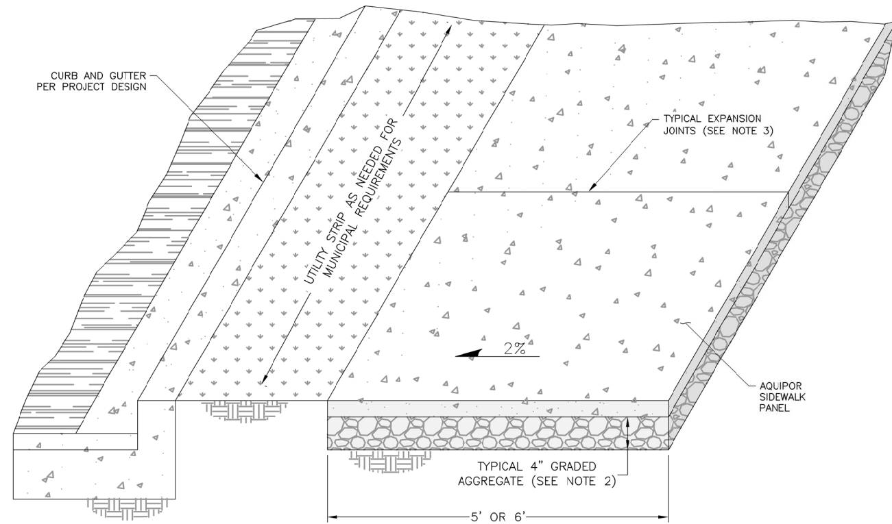
TYPICAL SIDEWALK PANEL INSTALLATION
